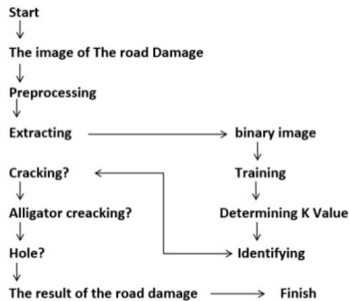
Fig. 3 Flow chart of image cclassification process.
